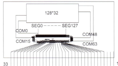
BLOCK DIAGRAM
