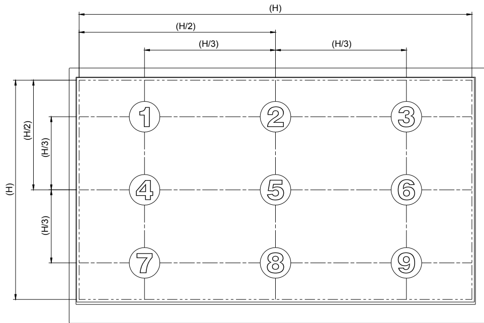
Fig.6-1 Measuring point
