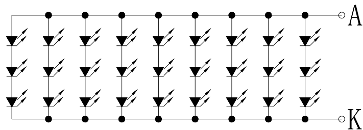
LED电路图 (3S9P=27LED)
